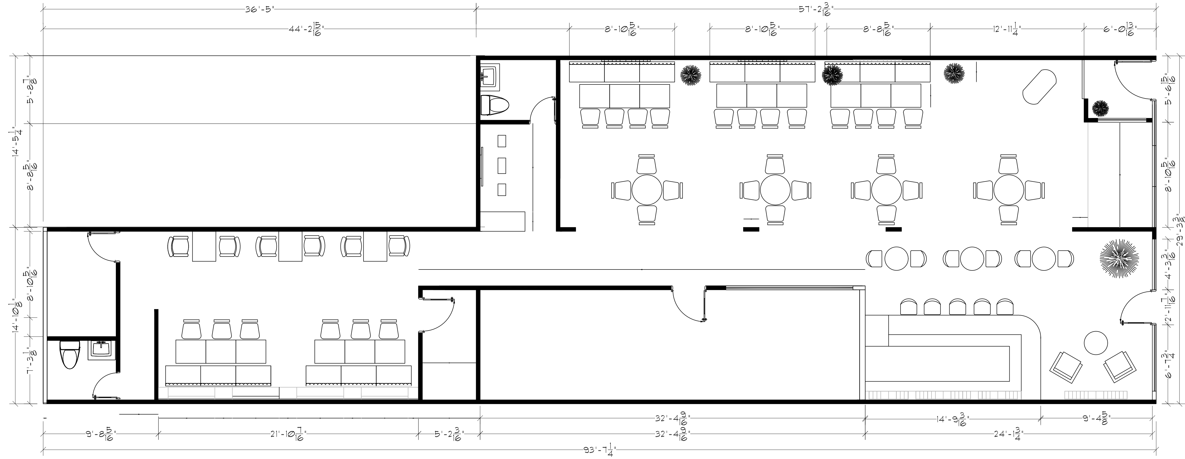
1 FP-1 PROPOSED FLOOR PLAN SCALE: 1/4" = 1'-0"
